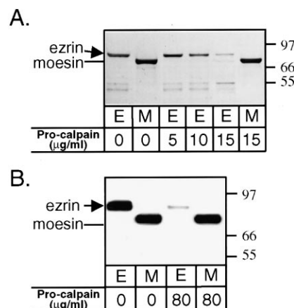
Fig. 3. Sensitivity of pure ezrin and moesin to calpain. Pure ezrin and moesin were separately incubated with pure pro-calpain and Ca^{2+} at \sim 22^\circ\text{C} for 20 min. A: Coomassie blue-stained gel shows ezrin (E) incubated with 0, 5, 10 and 15 \mu g/ml pro-calpain and moesin (M) incubated with 0 and 15 \mu g/ml pro-calpain. B: Immunoblot stained with a mAb that recognizes a shared epitope shows ezrin (E) and moesin (M) incubated with 0 and 80 \mu g/ml pro-calpain.
